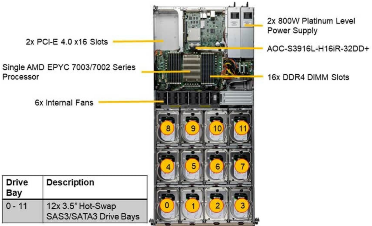
(Top View – System)
