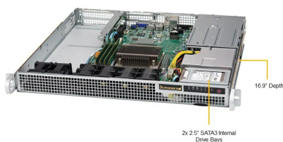
SuperServer SYS-1019S-WR (Angled View - System)
