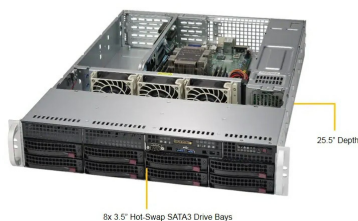
SuperServer SYS-5029P-WTR (Angled View - System)
