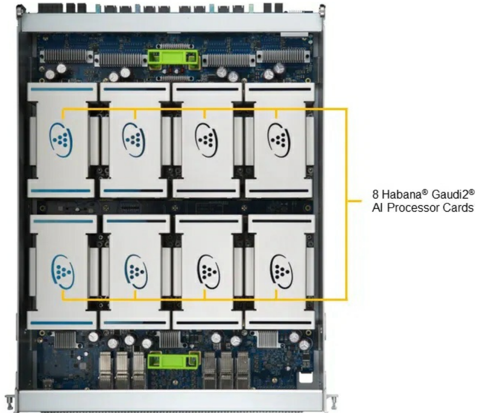
(Top View – Node)
