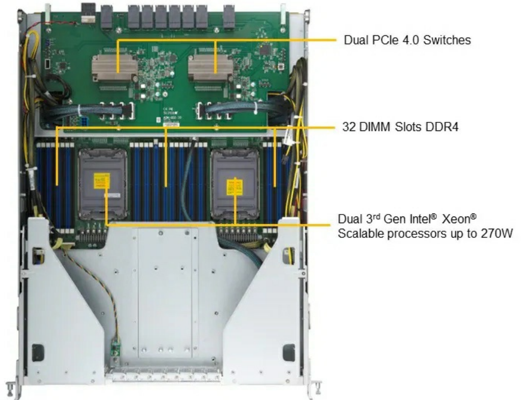
(Top View – Node)
